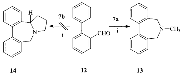
Scheme 5 Reagents and conditions: i, p -xylene, reflux.
